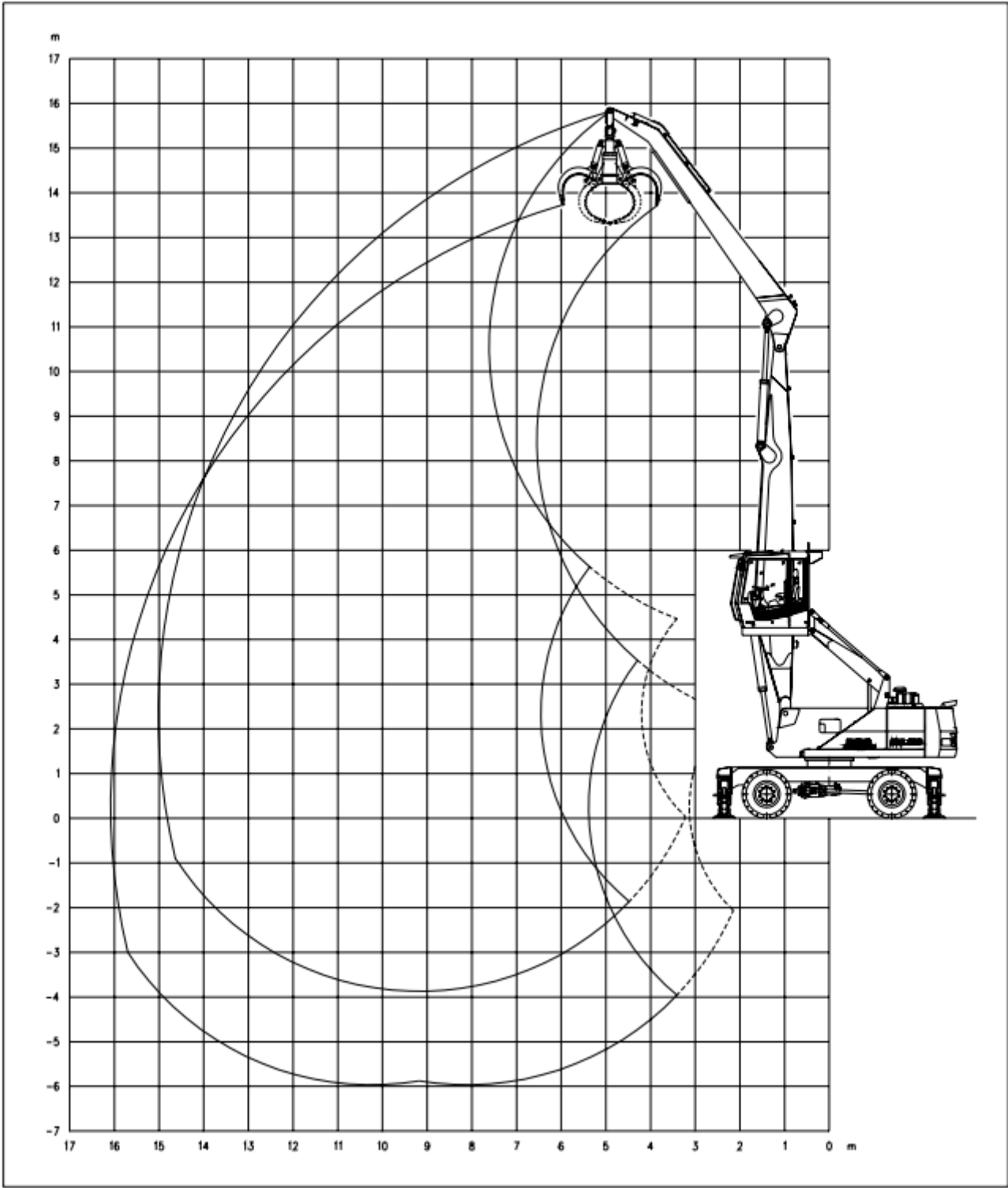
Fig. 9 Working range diagram (15 m loading equipment)
