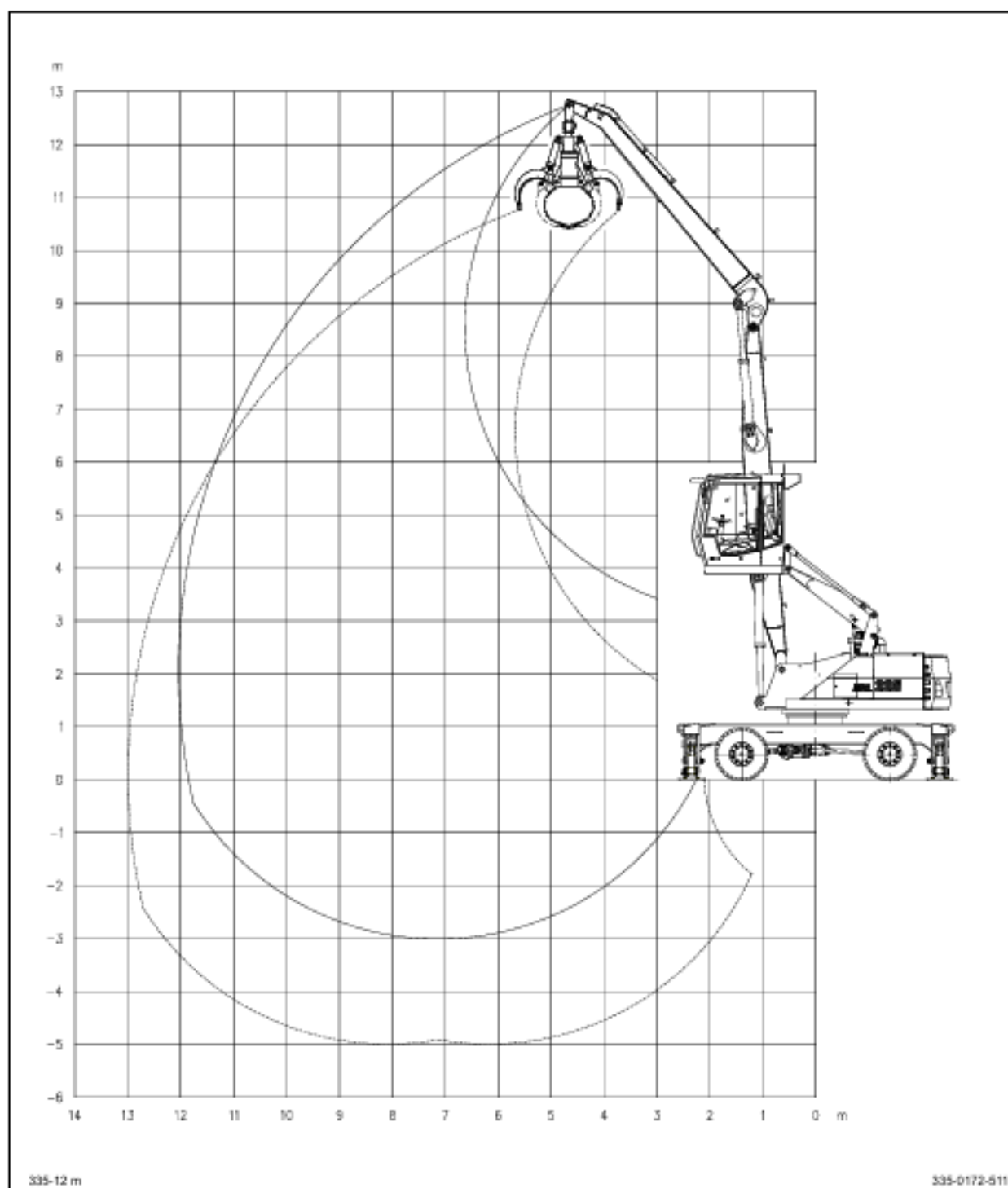
Fig. 10 Working range diagram (12 m loading equipment)
